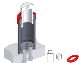
Easy Manifold+Abstreifring NV 5 NCS50-25-A-E-W
